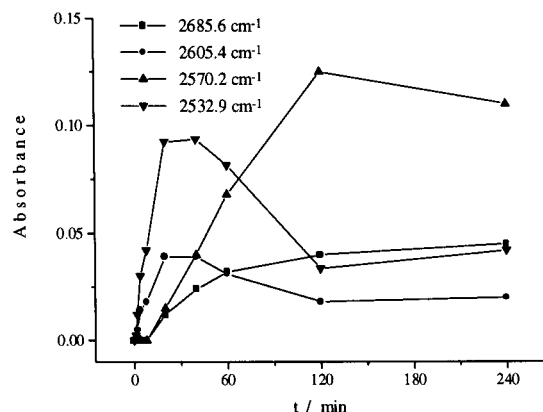
Figure 9. Plot of the \nu(\text{SH}) region in the IR spectrum of an Ar matrix initially containing diacetyl sulfide vs irradiation time.
