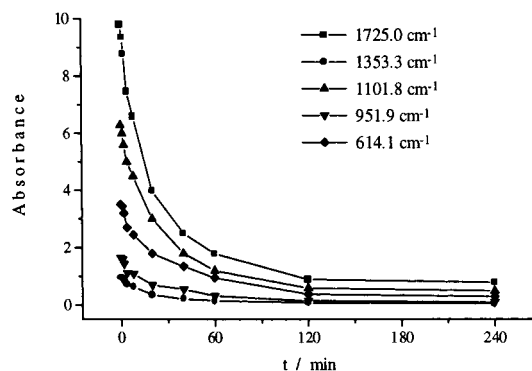
Figure 4. Plot of the intensities of the bands assigned to \text{CH}_3\text{C}(\text{O})\text{-SC}(\text{O})\text{CH}_3 in the IR spectrum of an Ar matrix initially containing diacetyl sulfide vs irradiation time.
