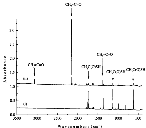
Figure 2. IR spectra of an Ar matrix containing \text{CH}_3\text{C}(\text{O})\text{SH} : (i) following deposition and (ii) after 240 min of broad-band UV–visible photolysis.
